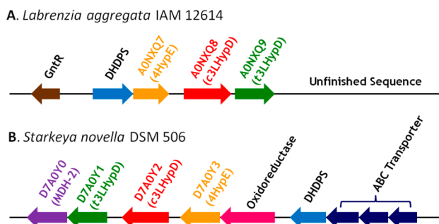
Figure 2. (A) Genome context of A0NXQ8 from L. aggregata IAM 12614. (B) Genome context of orthologous D7A0Y2 from Starkeya novella DSM 506. The genes encoding orthologues are highlighted with the same color. DHDPS, member of the dihydrodipicolinate synthetase superfamily.
