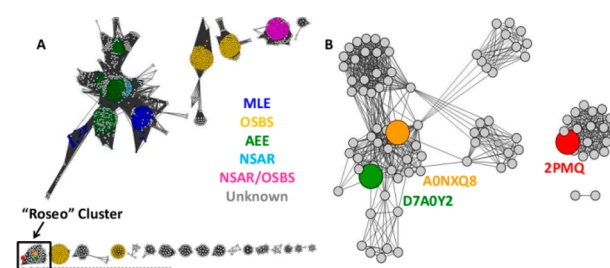
Figure 1. (A) SSN of the MLE subgroup displayed at a BLASTP e -value of 10^{-50} ; the “Roseo” cluster is boxed. (B) SSN of the “Roseo” cluster displayed at a BLASTP e -value of 10^{-80} ; 2PMQ, A0NXQ8, and D7A0Y2 are denoted by the red node, orange node, and green node, respectively.
